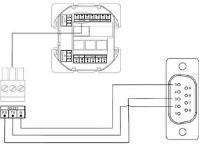
VLCPARS232 pin layout
