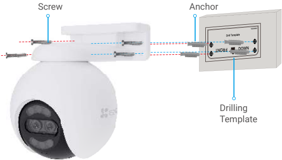
Fig. 2 Wall Mount
