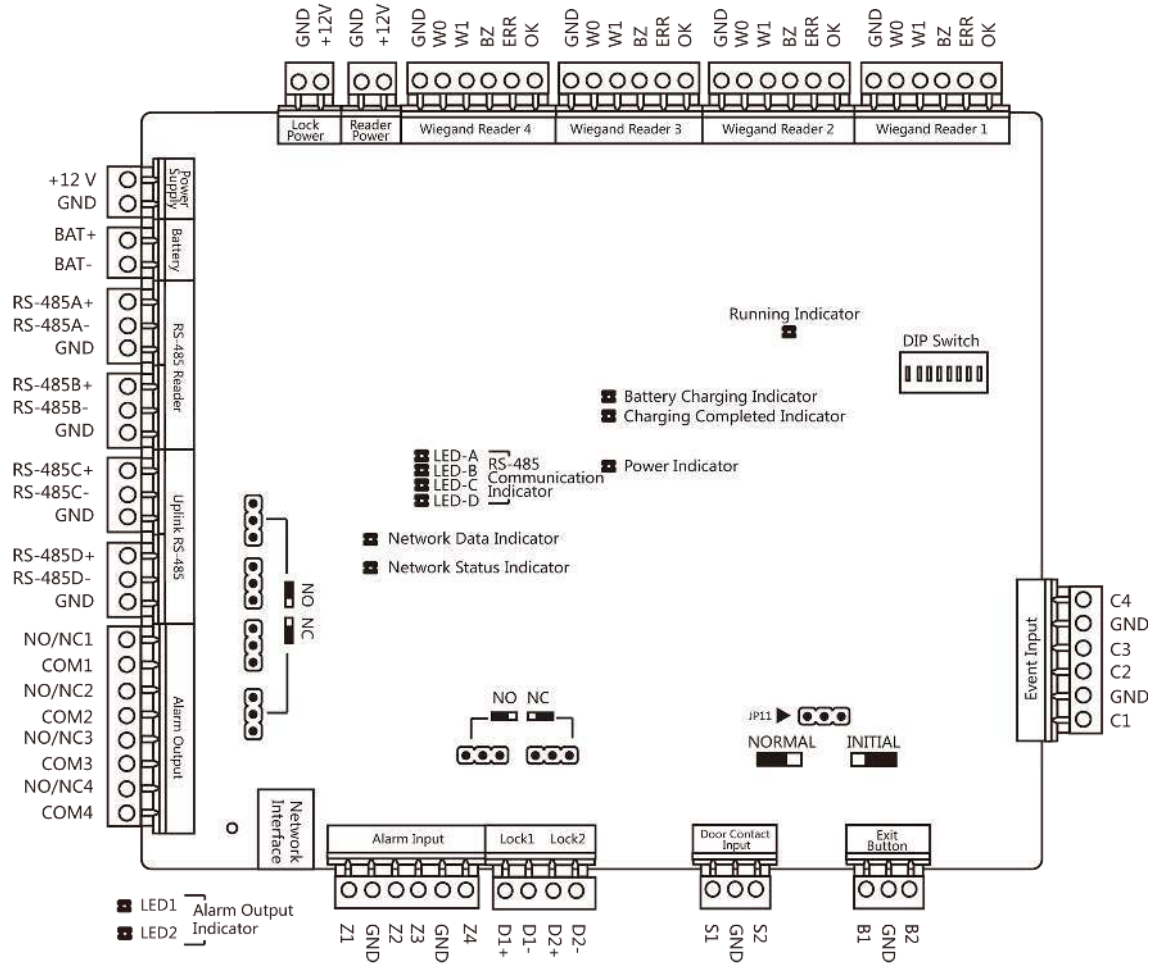
Figure 3-2 Two-Door Access Controller Main Board
