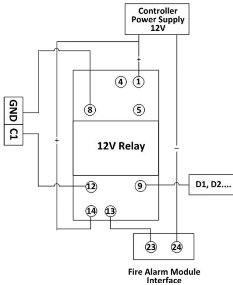
Figure 5-14 Fire Alarm Module Wiring
