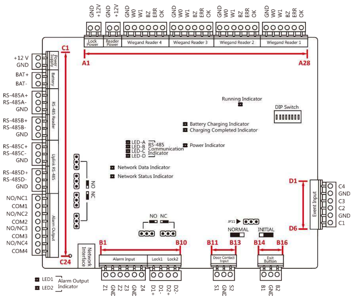
Figure 4-2 Two-Door Access Controller Main Board
