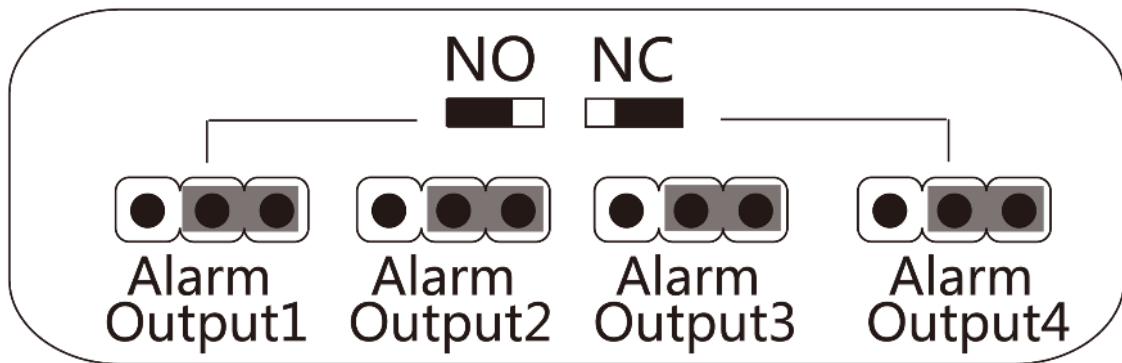
Figure 6-6 NC Status
