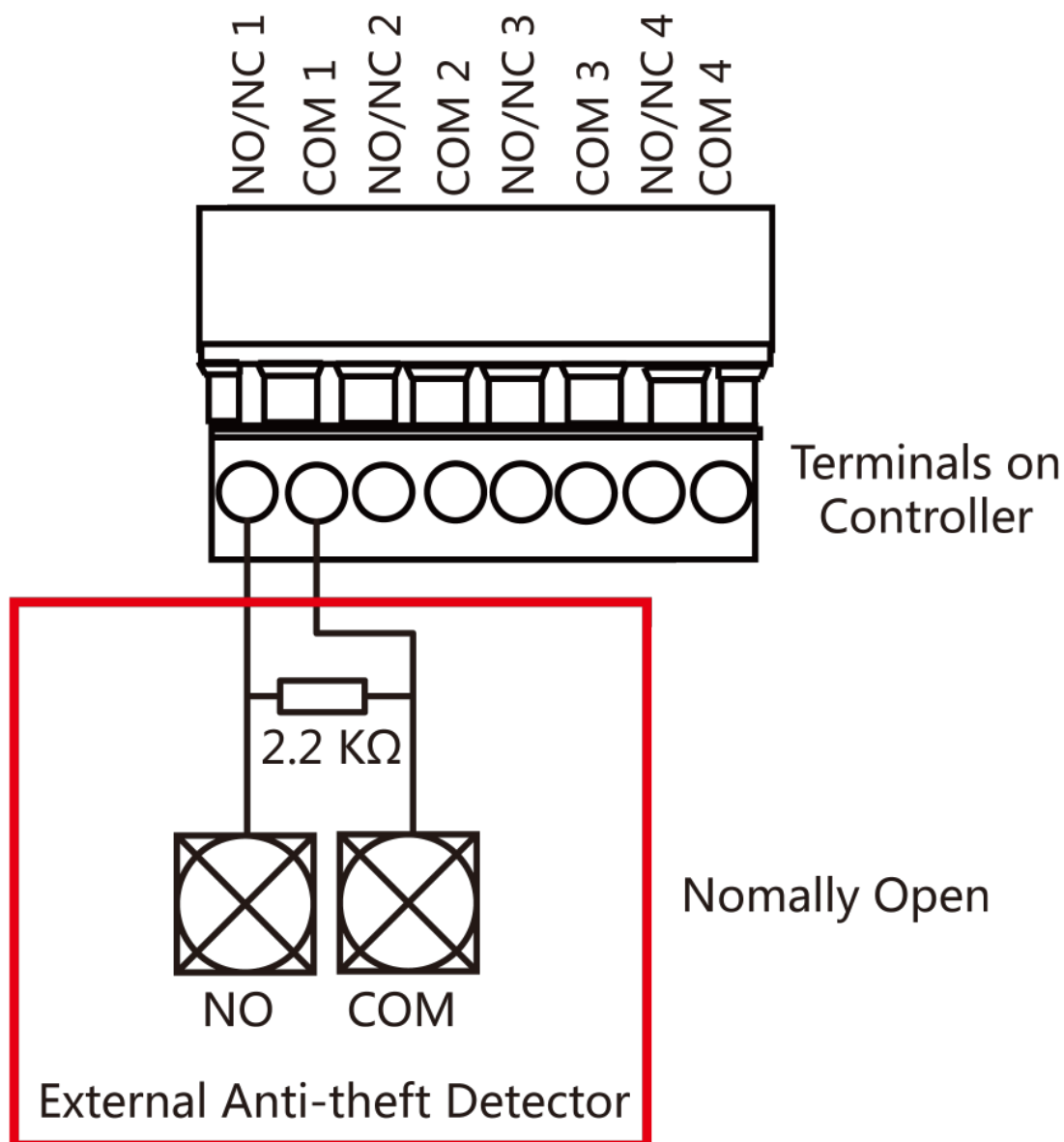
Figure 5-12 NO Wiring
