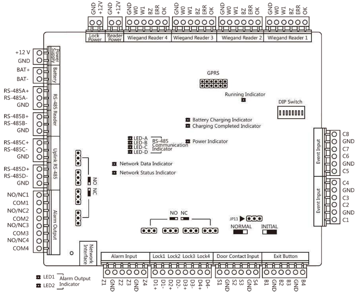
Figure 3-3 Four-Door Access Controller Main Board
