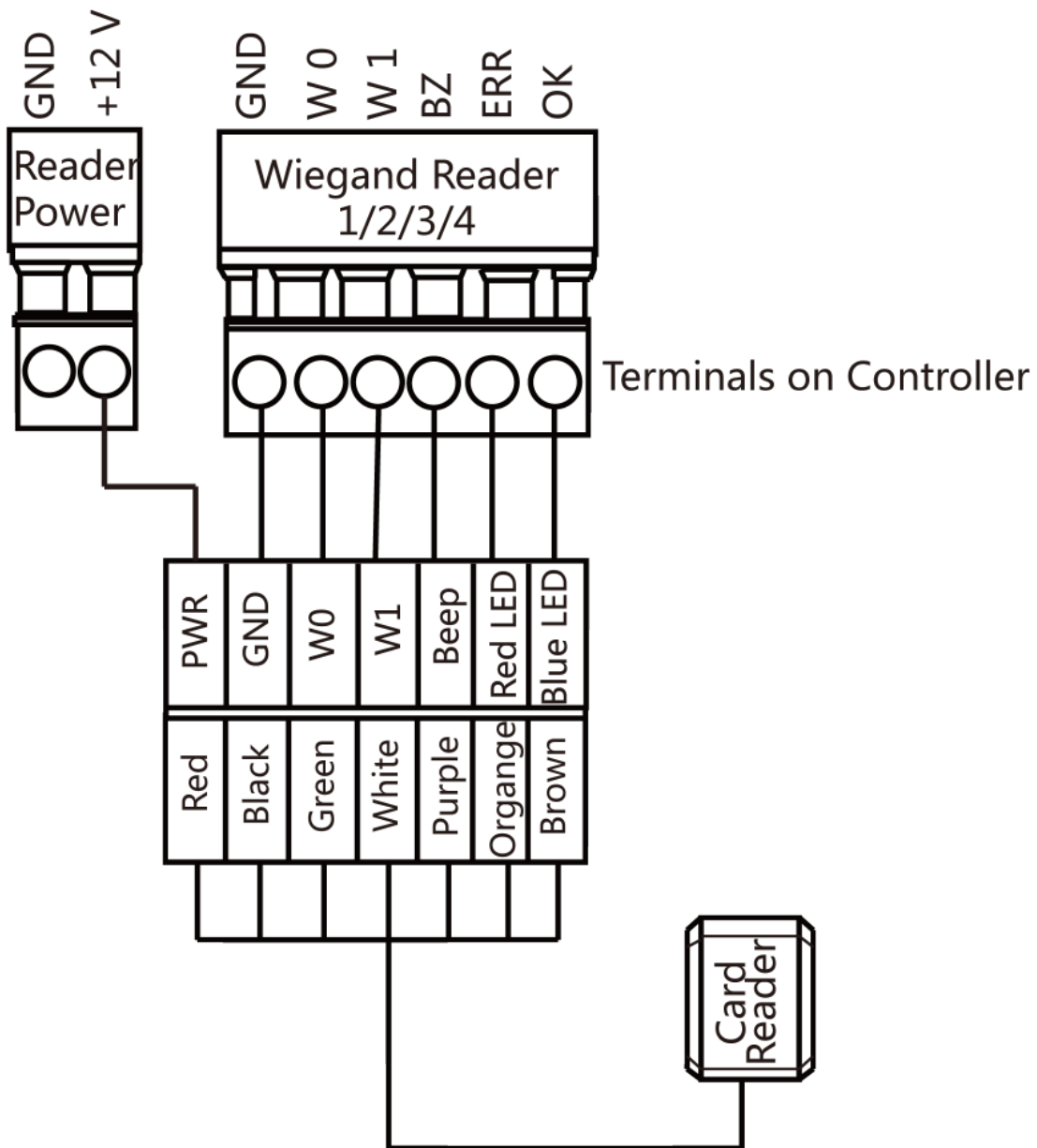
Figure 5-4 Wiegand Card Reader Wiring Diagram
