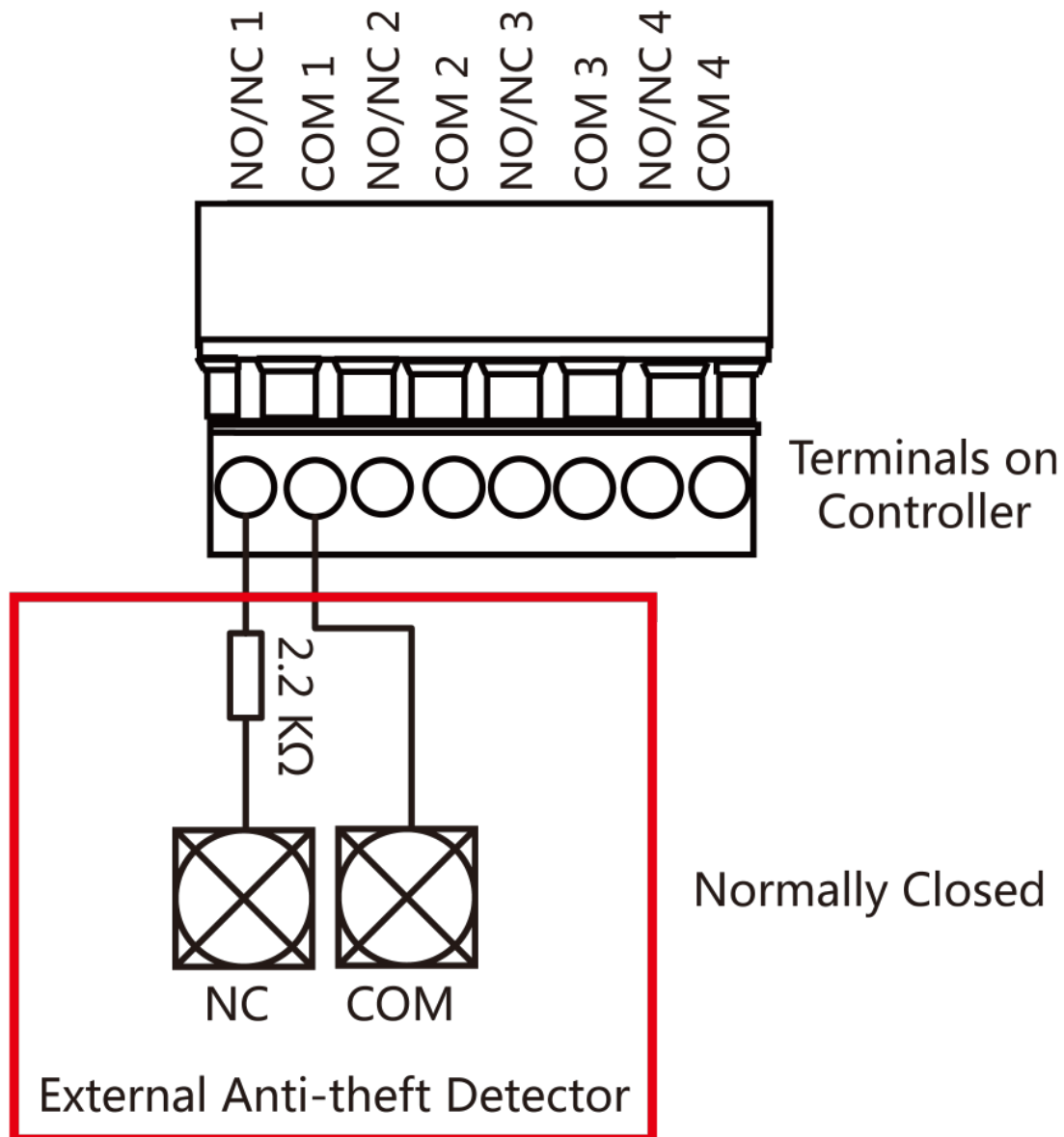
Figure 5-13 Normally Closed Wiring
