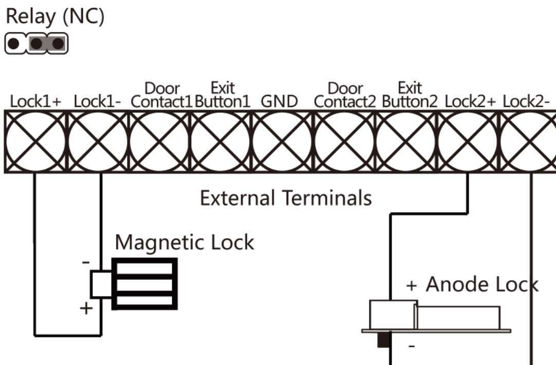
Figure 5-7 Wiring Diagram of Anode Lock
