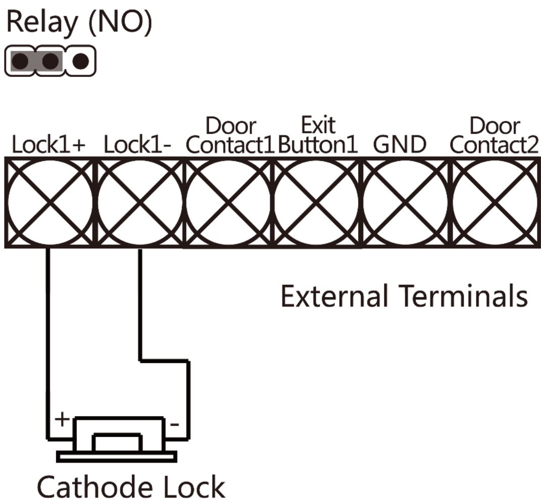
Figure 5-6 Wiring Diagram of Cathode Lock
