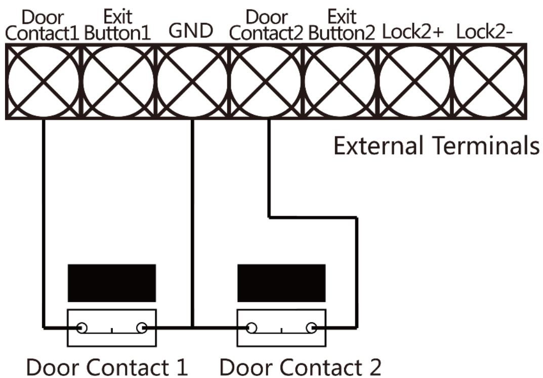
Figure 5-10 Door Contact Wiring
