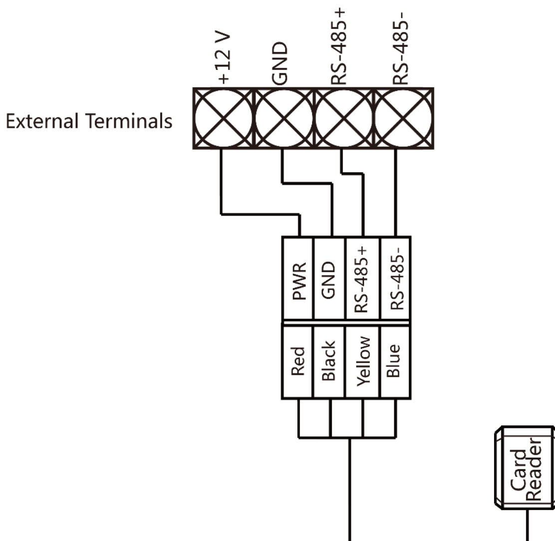
Figure 5-5 RS-485 Card Reader Wiring Diagram
