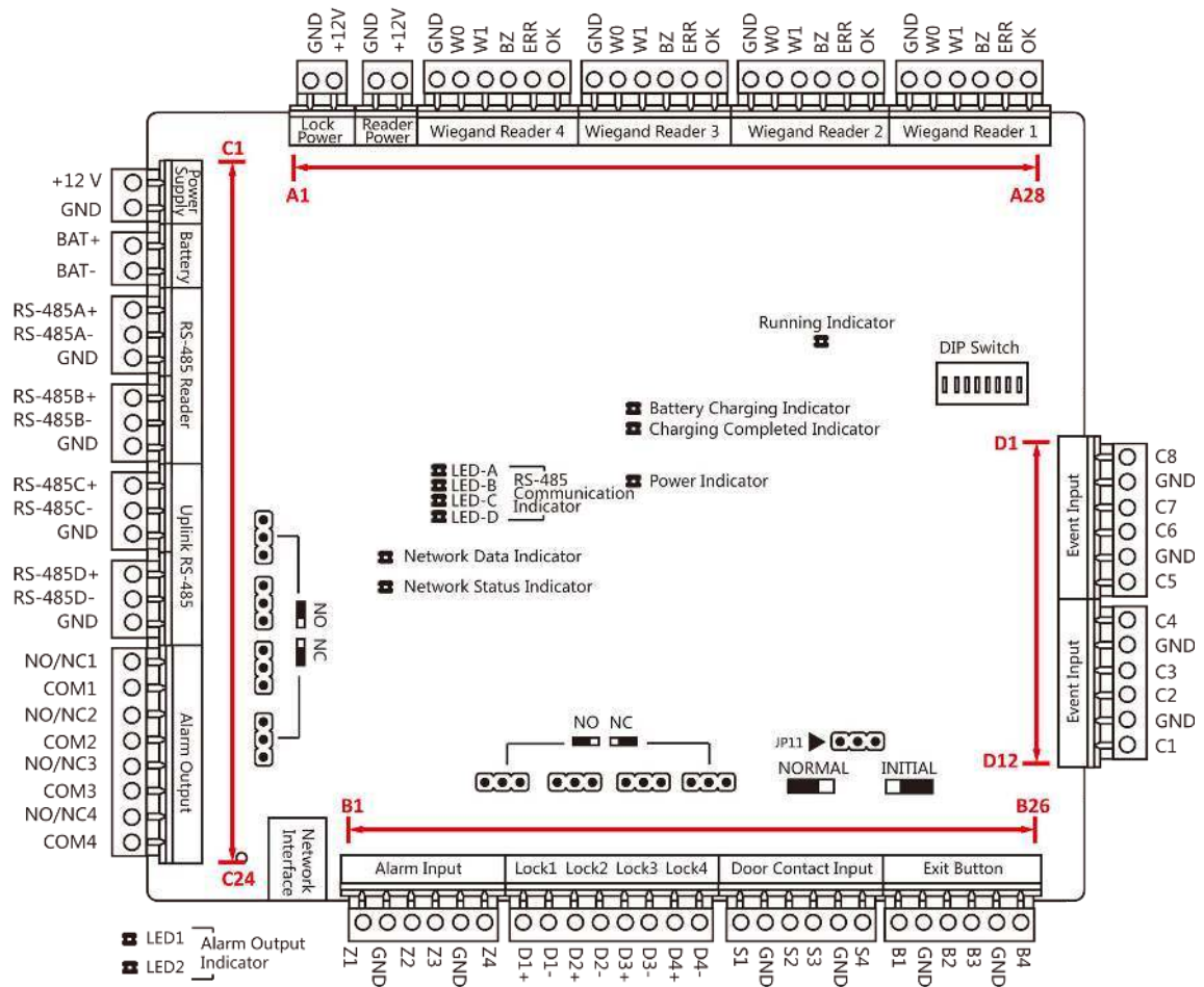
Figure 4-3 Four-Door Access Controller Main Board
