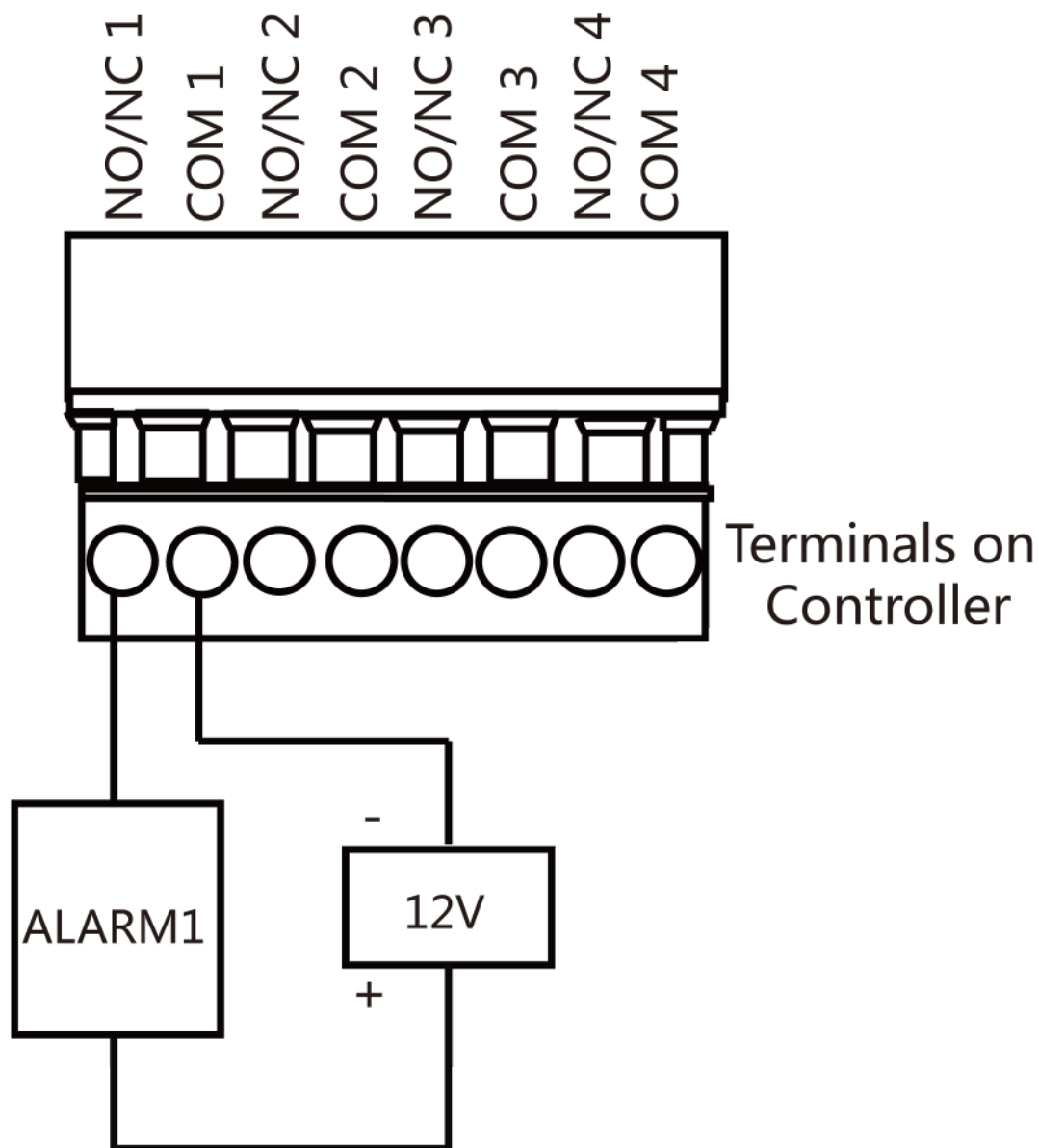
Figure 5-8 External Alarm Device Wiring
