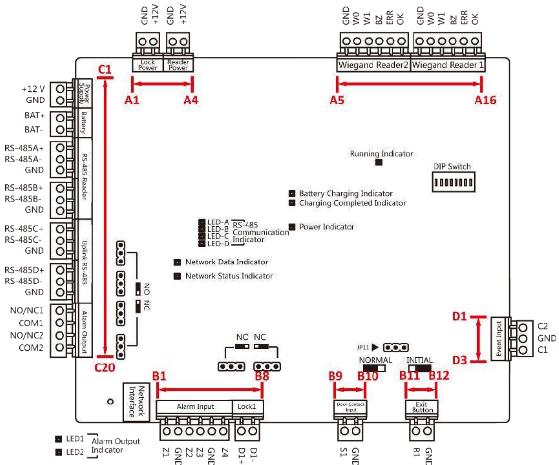
Figure 4-1 Single-Door Access Controller Main Board
