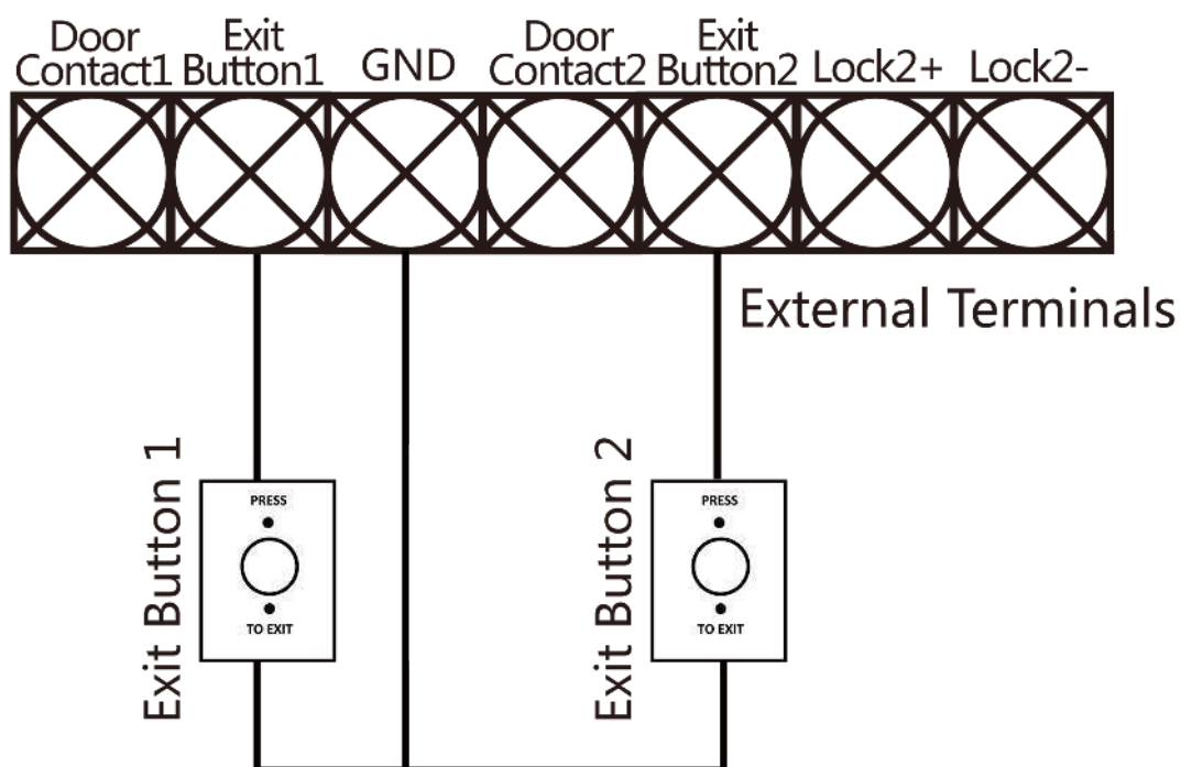
Figure 5-9 Exit Button Wiring
