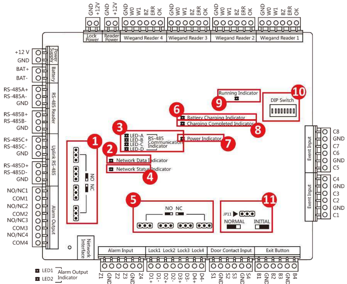
Figure 3-4 Four-Door Access Controller Component Diagram
