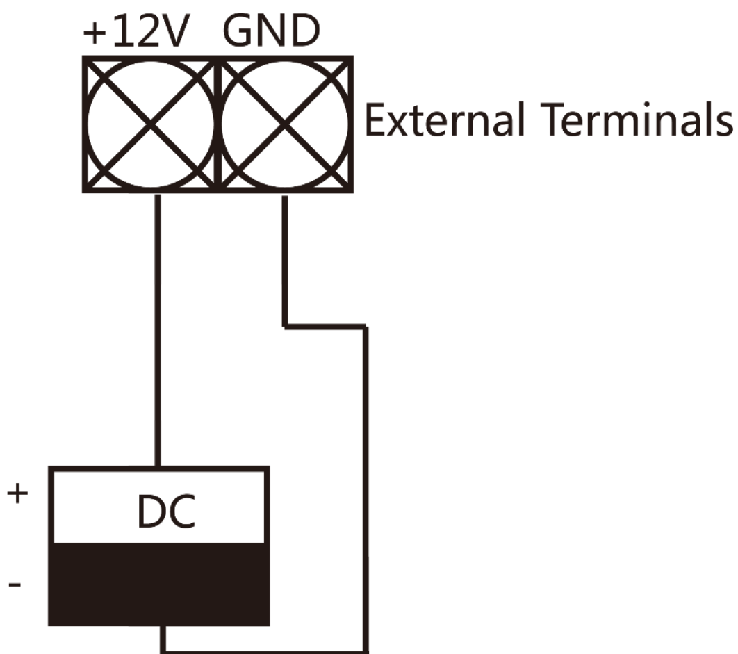
Figure 5-11 Power Supply Wiring
