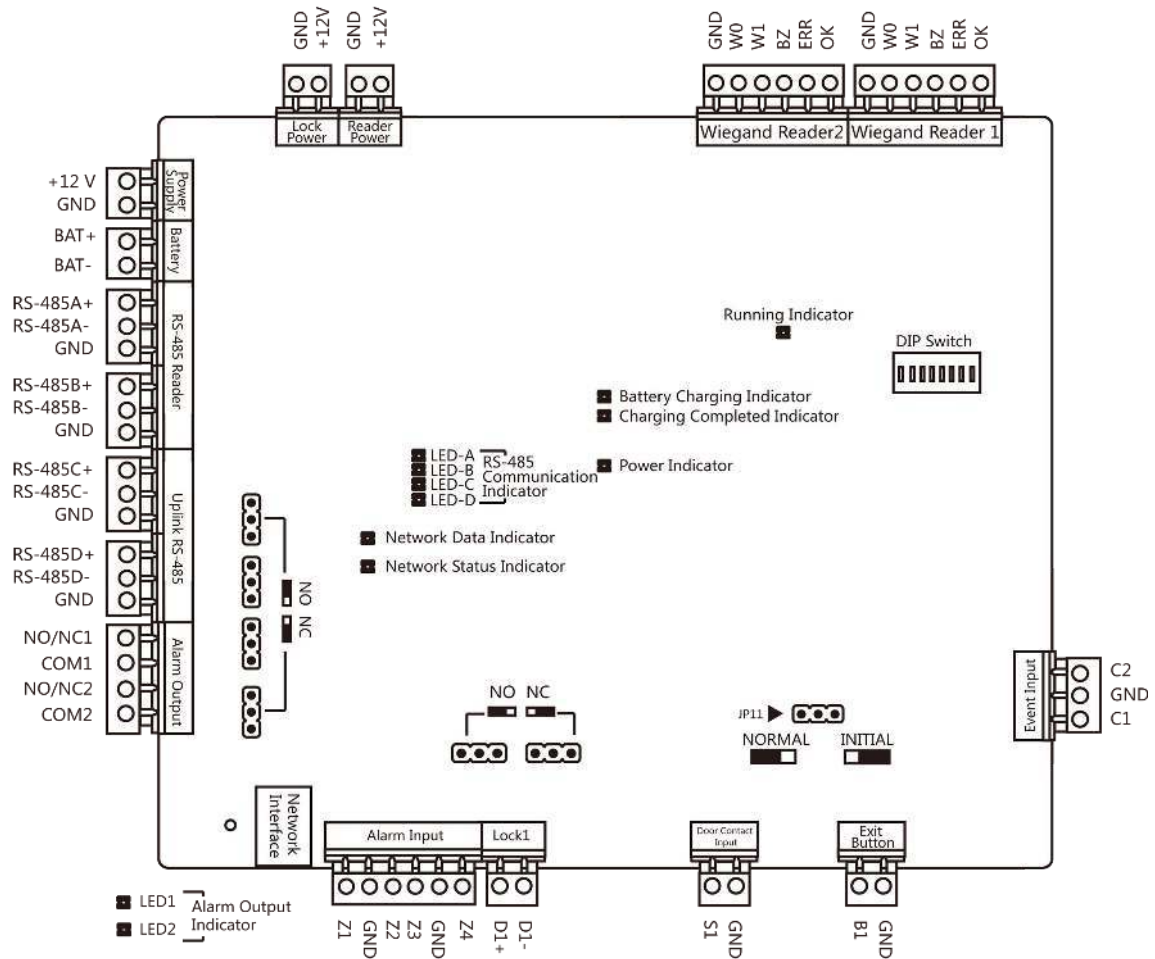
Figure 3-1 Single-Door Access Controller Main Board
