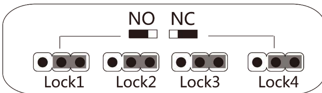
Figure 6-4 NC Status
