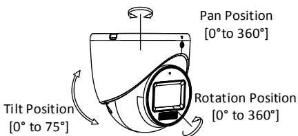
Figure 2-9 3-Axis Adjustment
