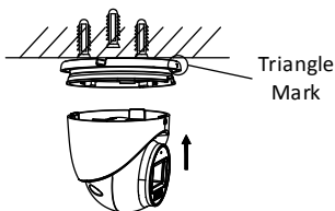
Figure 2-8 Install the Camera Back
