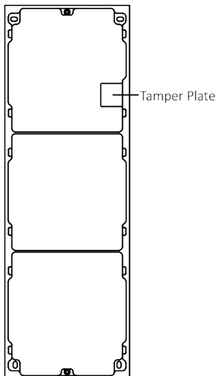
Figure 4-31 Mounting Frame
