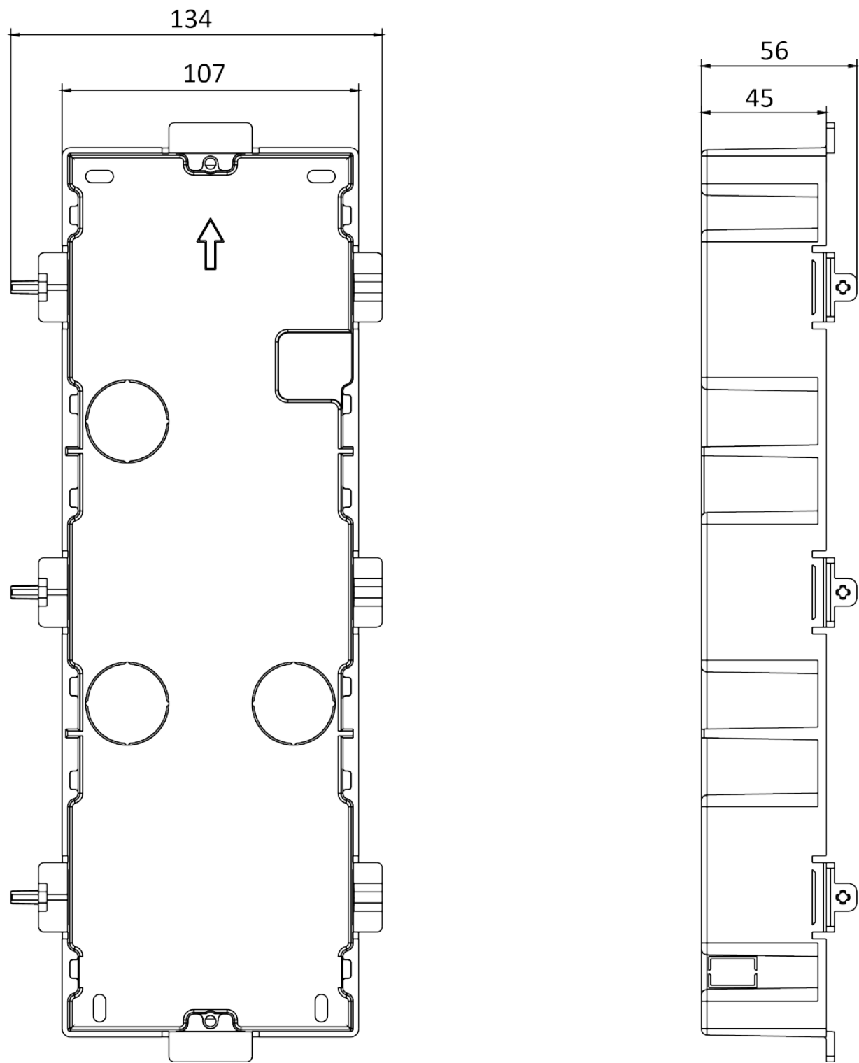
Figure 4-52 Gang Box
