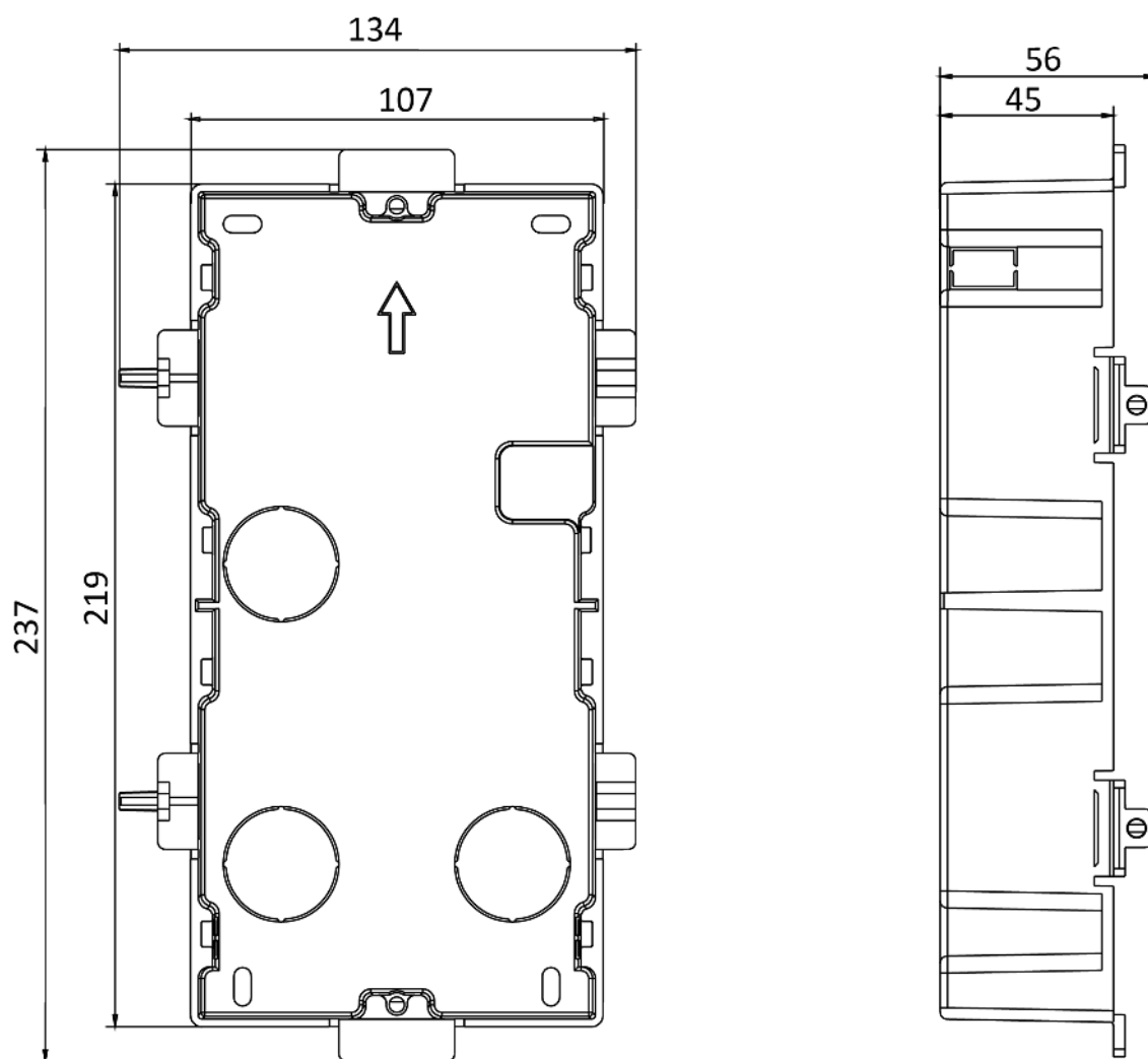
Figure 4-21 Gang Box
