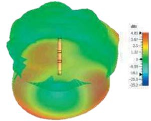
3D Plot Element D Top (5400 MHz)
