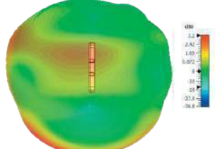
3D Plot Element D Top (2600 MHz)
