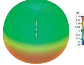
3D Plot Element C Top (750 MHz)
