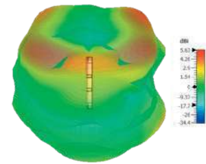
3D Plot Element C Top (5400 MHz)
