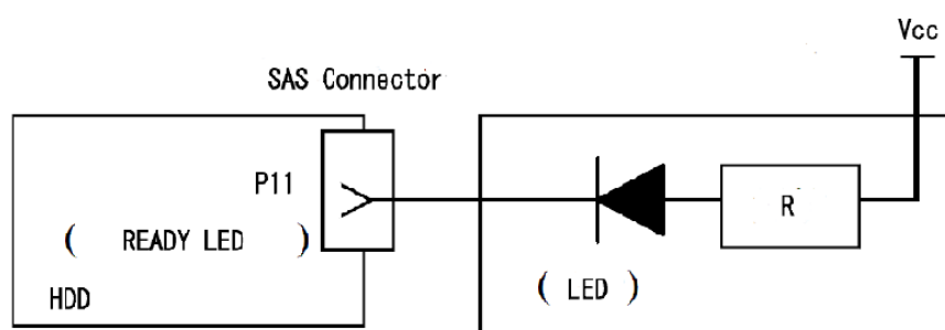
Figure 4.9 Recommended external circuit for Ready LED output
