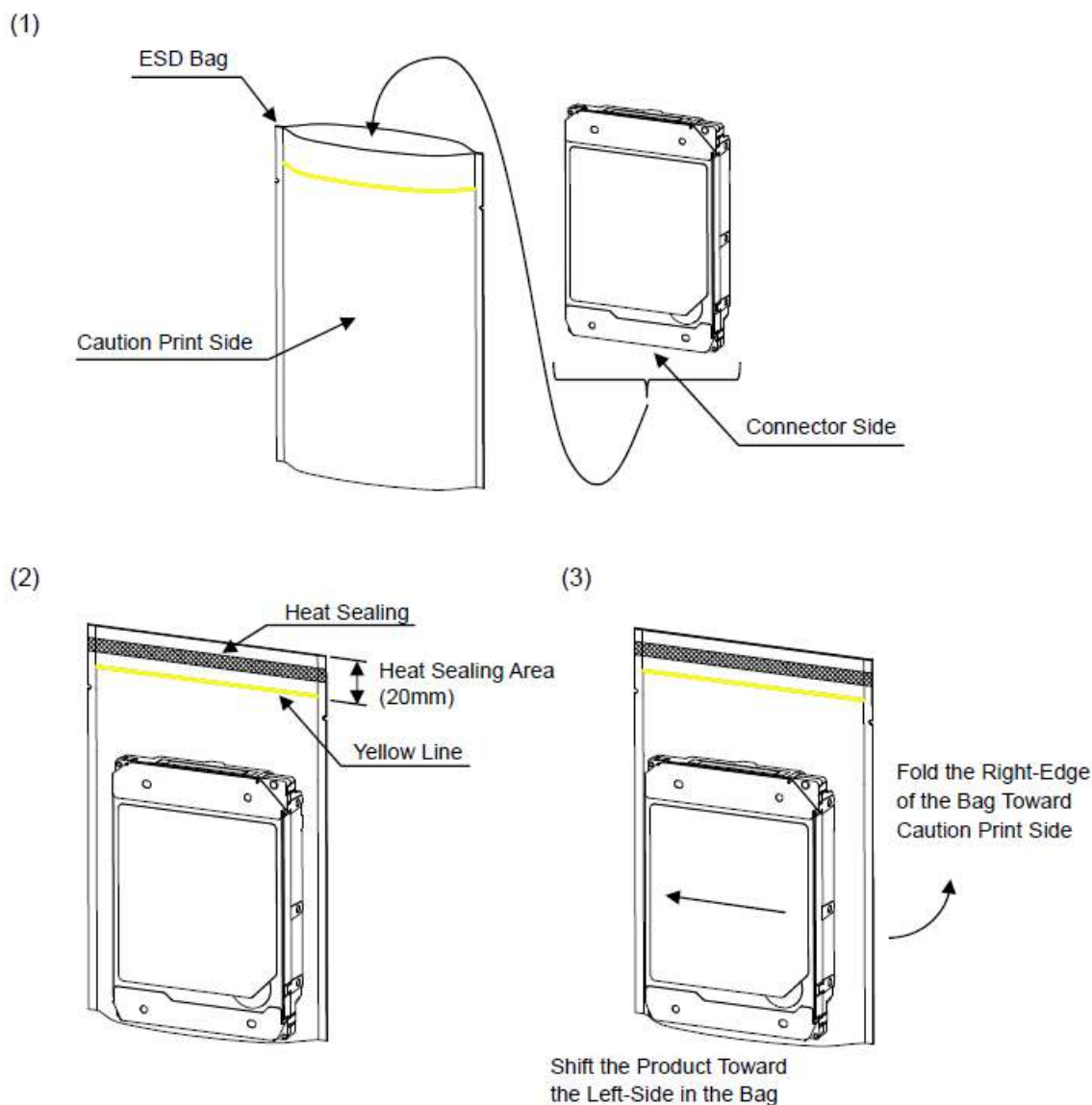
Figure 6.2 Bag packaging
