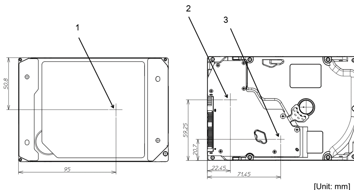
Figure 4.5 Surface temperature measurement points
