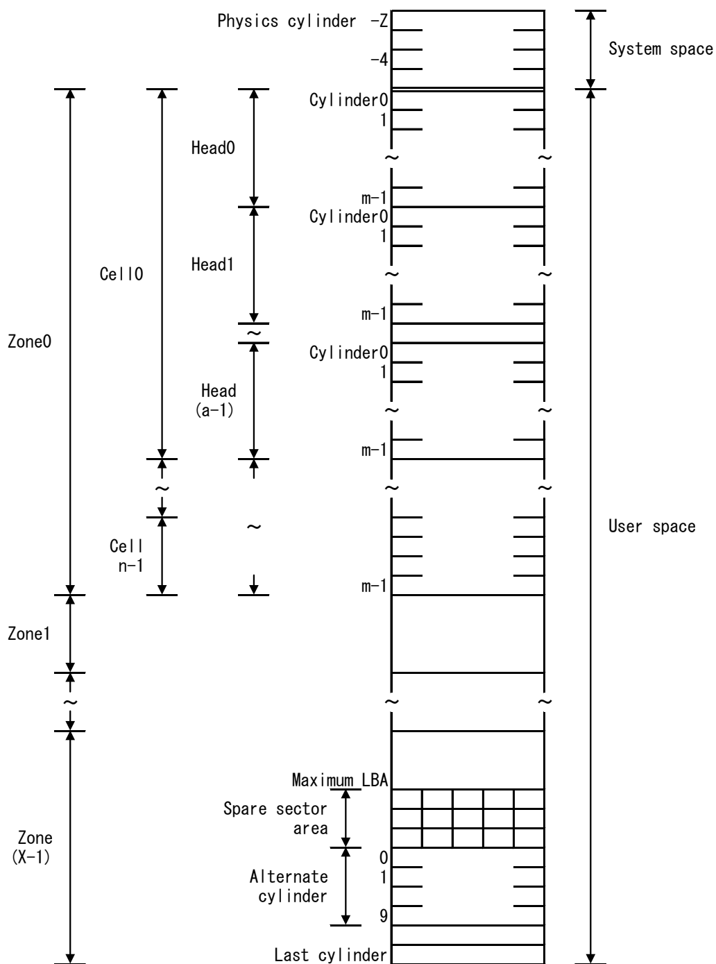
Figure 3.1 Cylinder configuration
