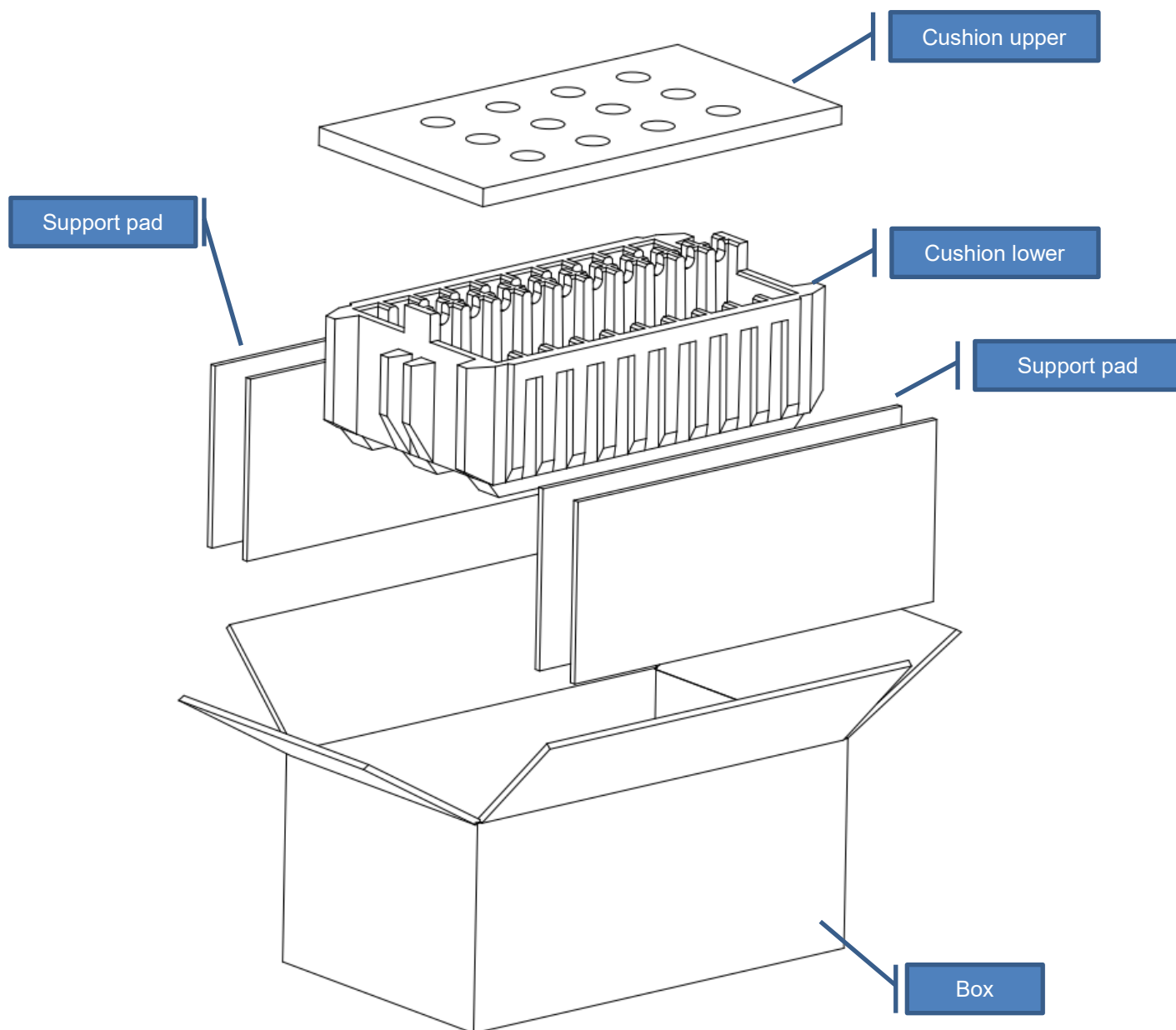
Figure 6.3 Box packaging
