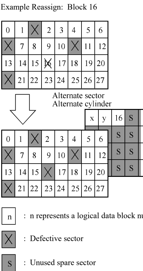
Figure 3.7 Alternate block allocation by REASSIGN BLOCKS command
