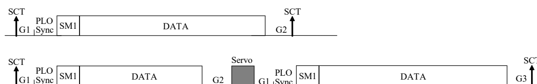
Figure 3.5 Sector format
